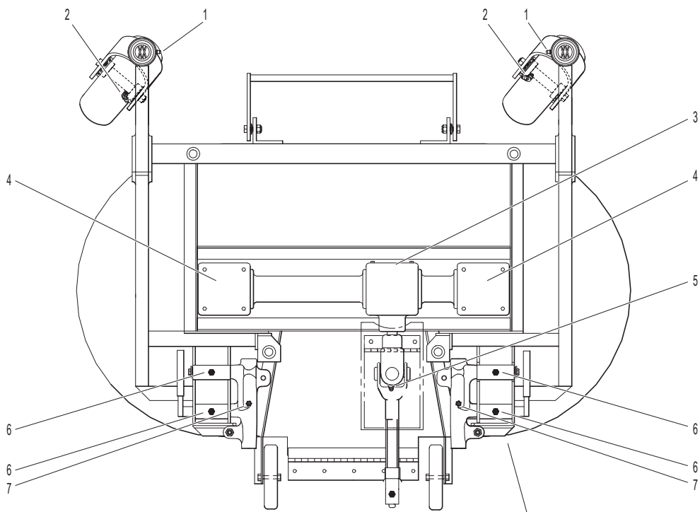
36", 42", 48" & 52" Assemblies
