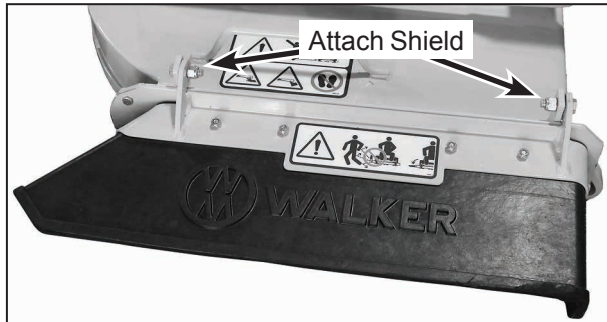
Discharge Shield Installation on Side Discharge Deck
