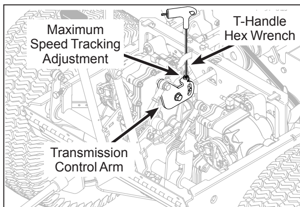
Maximum Speed Tracking Adjustment (Shown with Parts Removed for Clarity)
