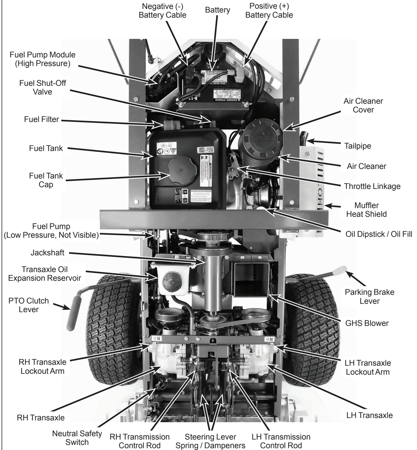
Top View (Body Raised)
