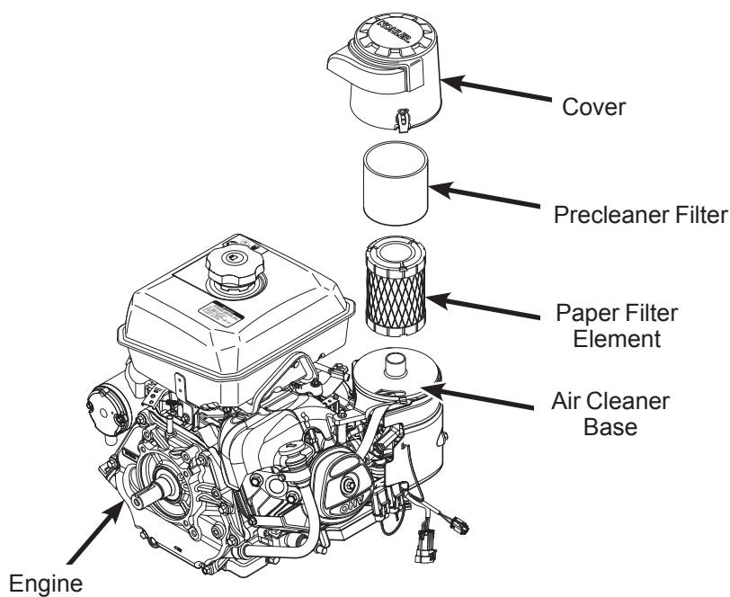
Engine Air Cleaner System Components
