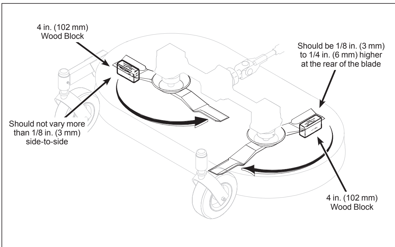
Deck Leveling
